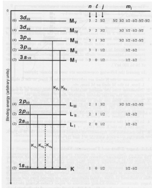
Typical energy level diagram for a high-Z atom showing sub-shell structure for K, L and M shells. Allowed (solid lines) and forbidden (dashed lines) K_{\alpha} and K_{\beta} transitions are also shown. Numbers in parentheses indicate maximum number of electrons in that sub-shell, 2j + 1 . (From Podgoršak, Fig. 3.1.)
